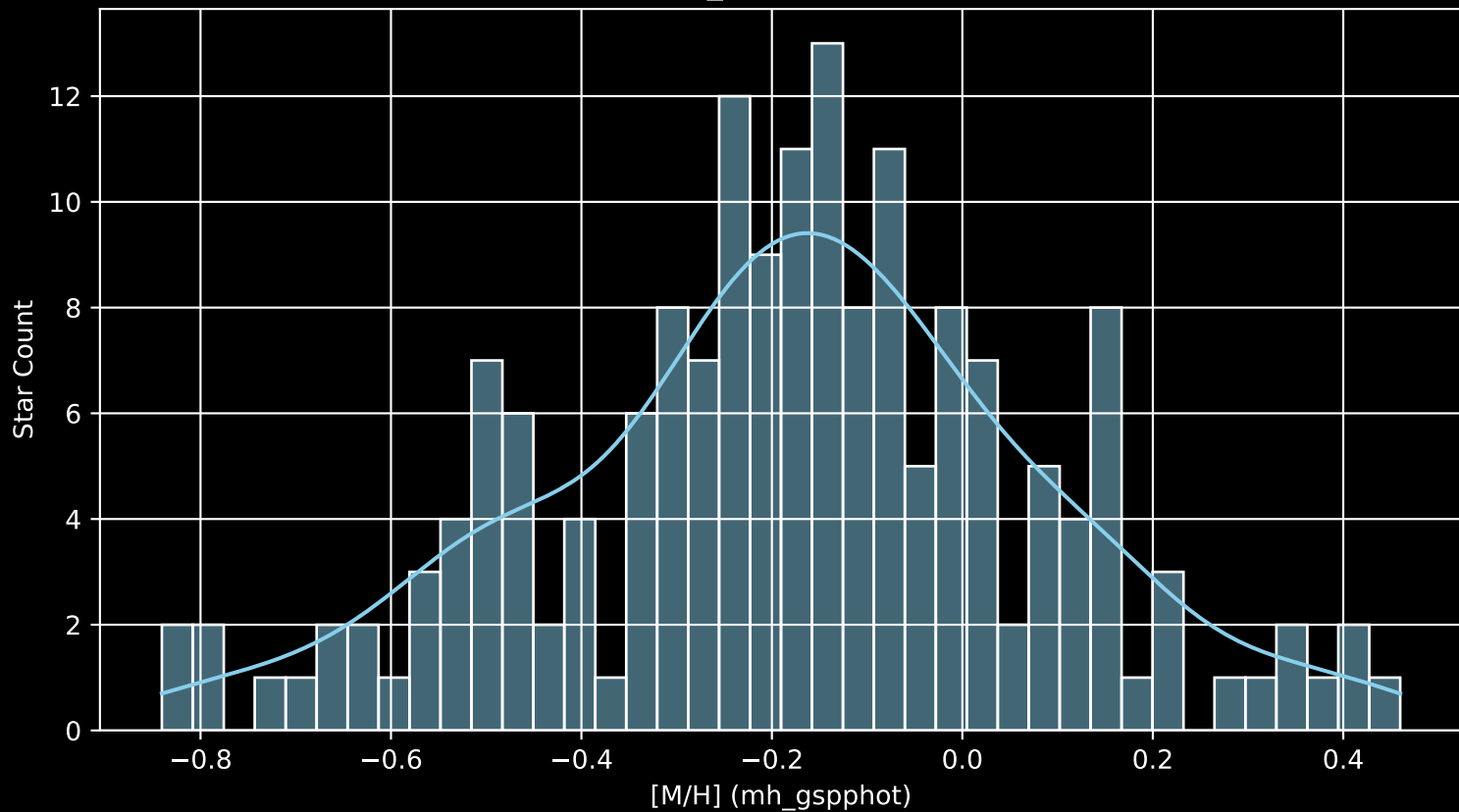
APOGEE DR17 Field: [CVZTILE_093+37_btx [M/H] (mh_gspphot) (n= 174)
