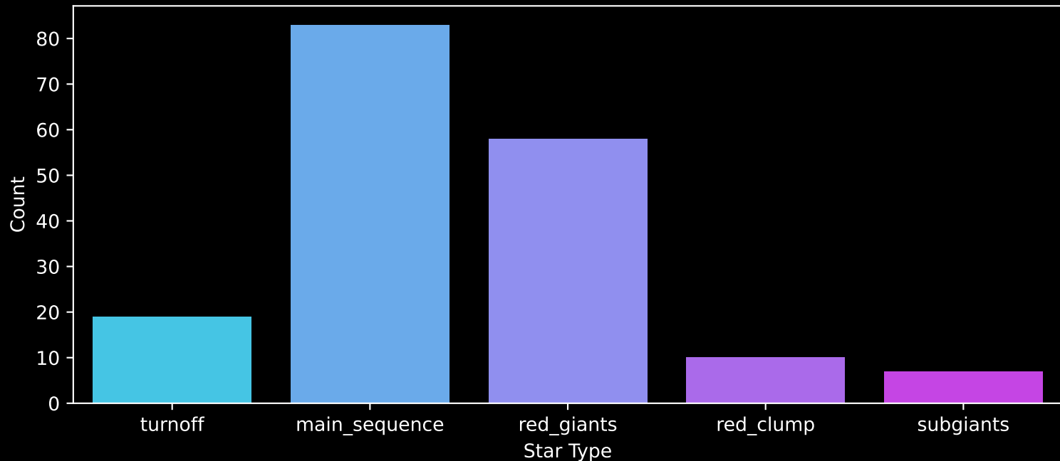
APOGEE DR17 Field: [CVZTILE_093+37_btx] Count plot of Star Type
