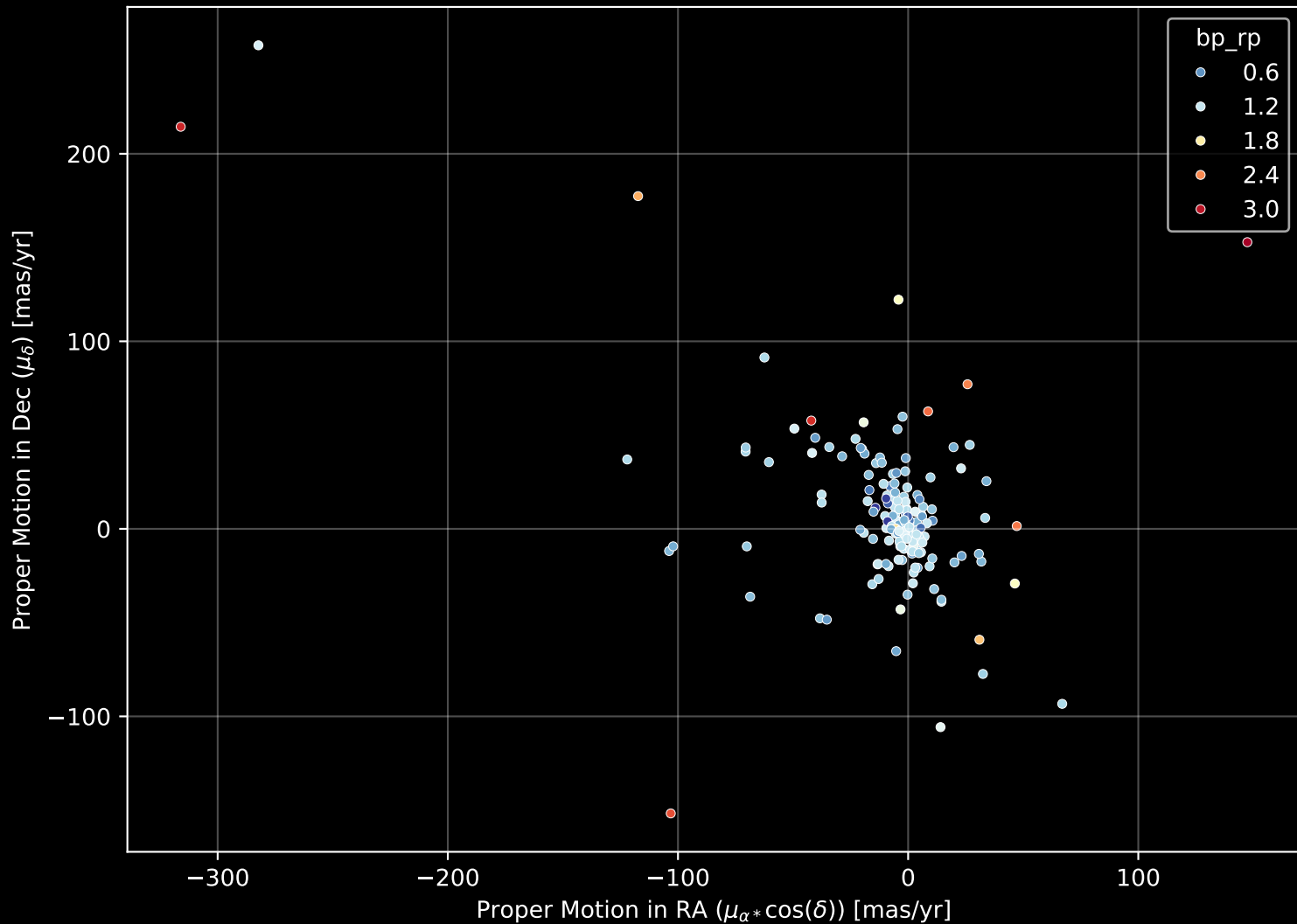
APOGEE DR17 Field: [CVZTILE_093+37_btx] Proper Motion Diagram (n= 177)
