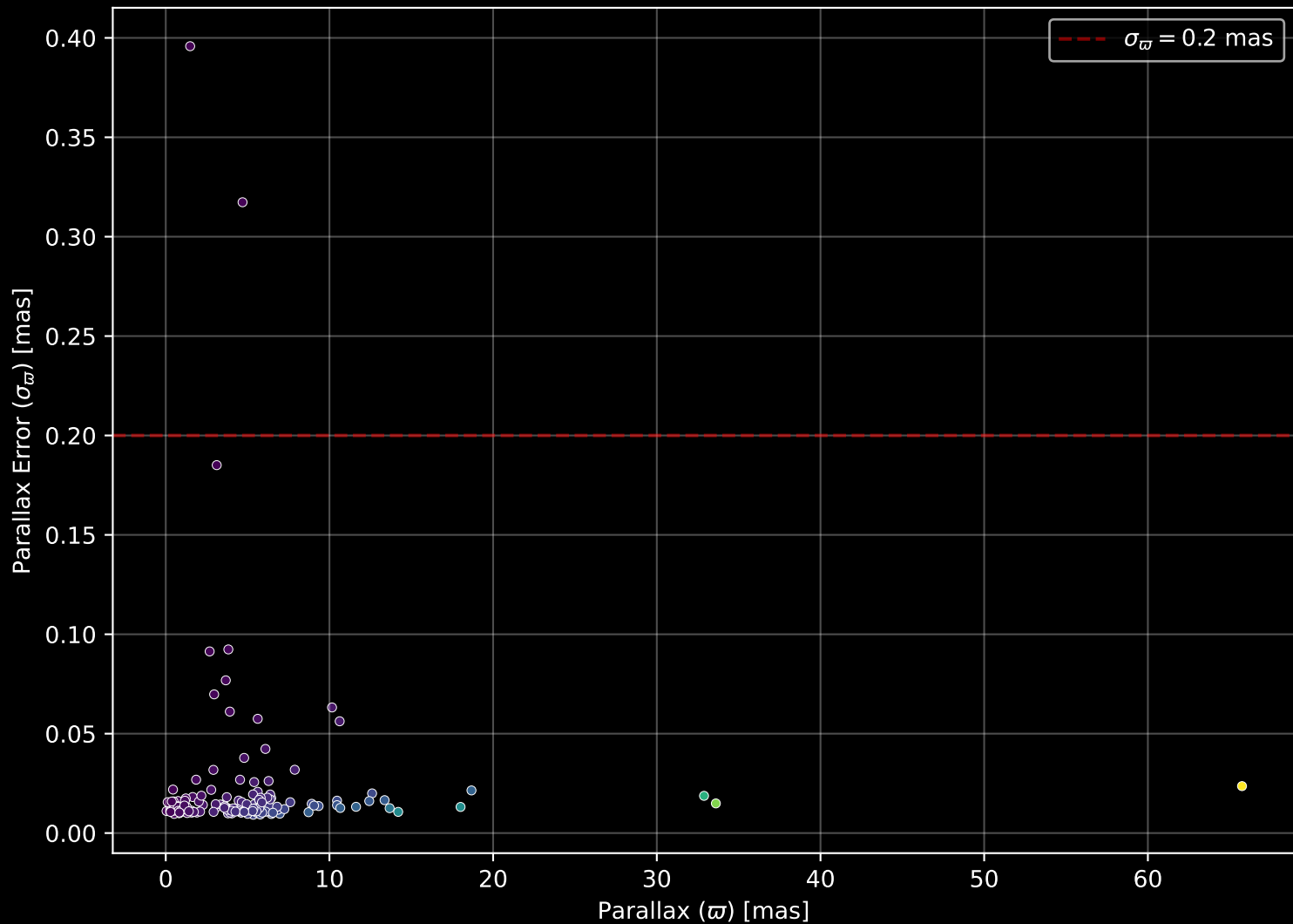
APOGEE DR17 Field: [CVZTILE_093+37_btx] Parallax Quality (n= 177)
