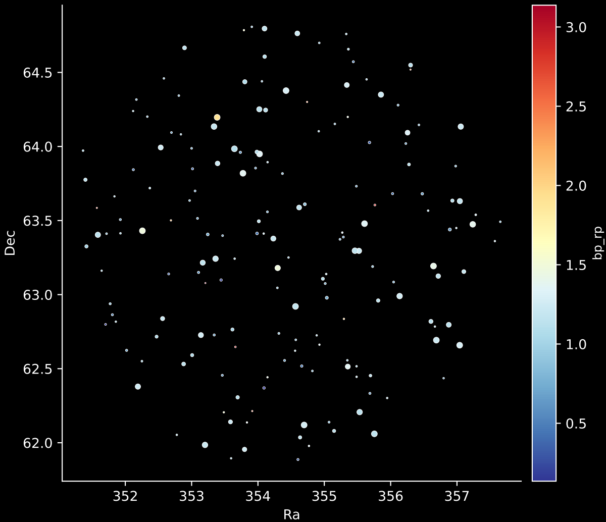
APOGEE DR17 Field: [CVZTILE_093+37_btx] Stars: 177
