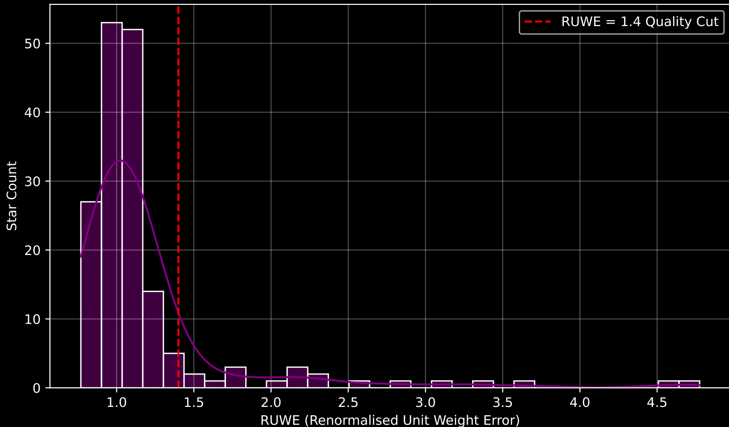
GAPOGEE DR17 Field [CVZTILE_093+37_btx] RUWE Distribution (n= 170)
